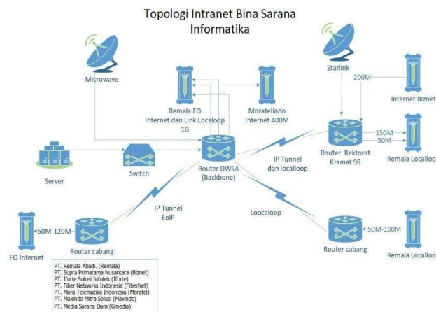
Gambar 2.53. Topologi Intranet UBSI
